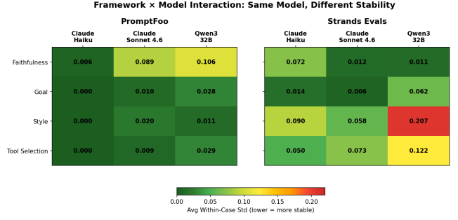
Figure 1: Avg within-case std by (evaluation harness × judge model) for each framework. PromptFoo (left) is uniformly stable. Strands (right) shows higher variance, with Qwen3/style as the only unstable cell.
