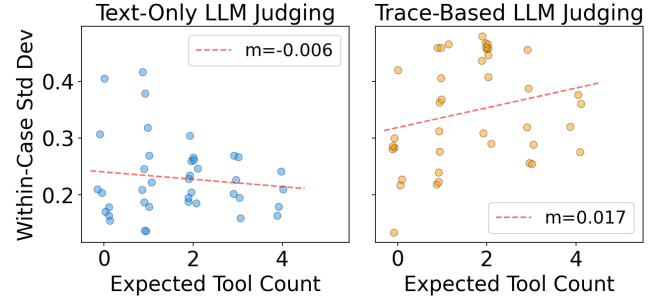
Figure 2: Within-case std dev vs. tool count (pooled).
