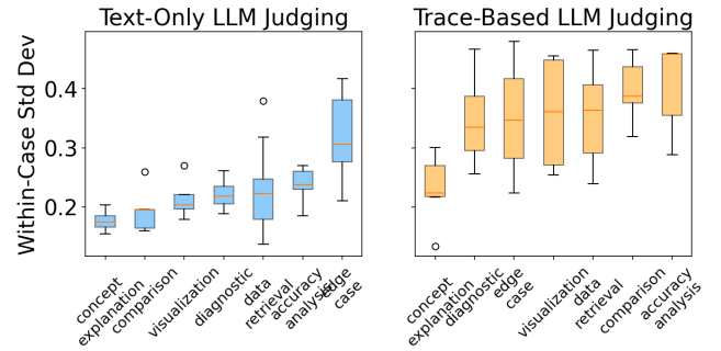
Figure 3: Within-case std dev by case category (pooled).
